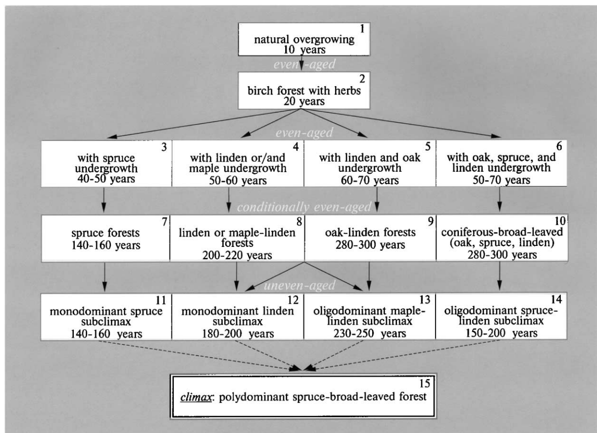
Fig. 1. Ideal course of succession through forest types (after-tillage series) in the Prioksko-Terrasnyi Biosphere Reserve, Moscow Region, Russia.
